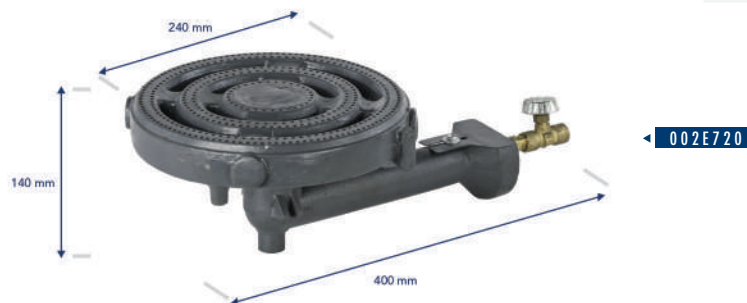
Model 50 LP gas burner
